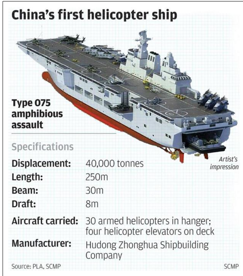
Figure 15. Type 075 LHD Unofficial artist’s rendering
