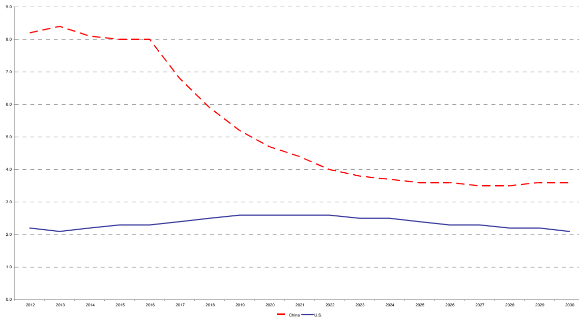
Figure 3. Projections of U.S. and Chinese Annual Real GDP Growth: 2012-2030 %
